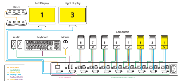
Figure 4: 2 RCUs cascaded for 8-port source selection on each display
