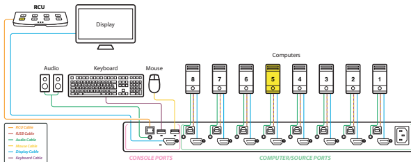
Figure 3: RCU connected to an 8-Port KVM Switch
