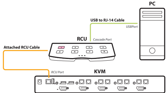
Figure 7: The RCU connected to a PC and KVM device, ready for programming.
