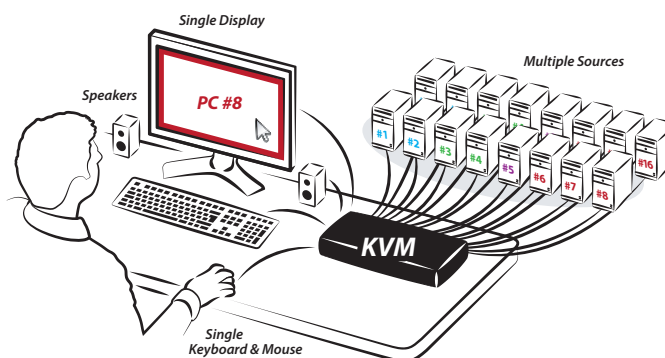
HSL Single-Head 16-Port KVM Switch System Diagram
