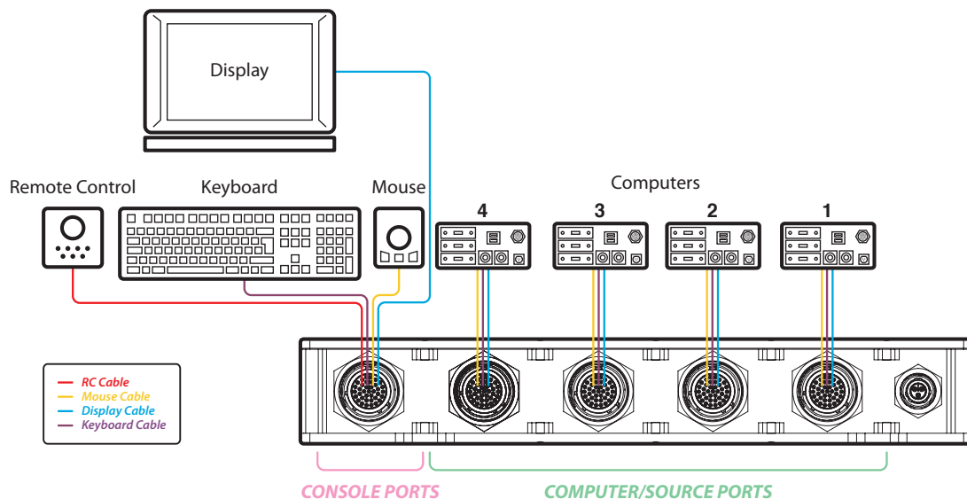
HSL Secure SK41D-4TR System Diagram
