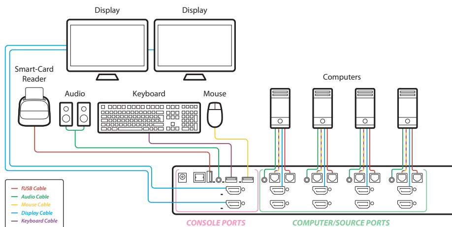
HSL Dual-Head 4-Port Secure KVM Switch System Diagram
