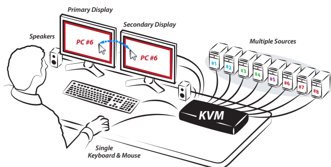
HSL Dual-Head 8-Port KVM Switch System Diagram
